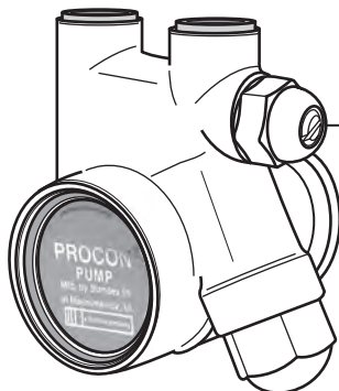
700008/F 150 Lt/h CON FILTRO WITH FILTER
