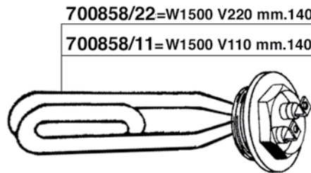
700858/22=W1500 V220 mm.140
