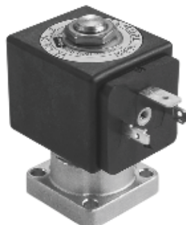
PARKER \varnothing 2,5 634294/22 V220/50/60 634294/11 V110/60
